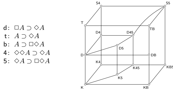
Fig. 1. Left: Some standard modal axioms
