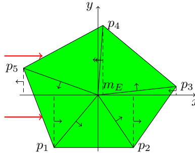
Figure 2: The mesh \mathcal{T}_E with a constant velocity
