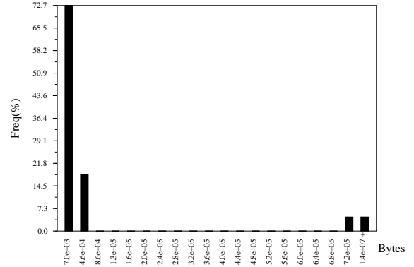
Fig. 4. PerDiS: size frequency, in bytes, of strongly connected components
