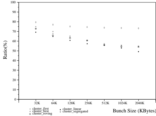
Fig. 9. PerDiS: proportion of inter-bunch references
