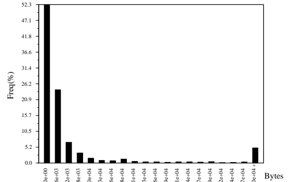
Fig. 1. PerDiS: object size class frequency distribution
