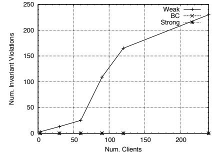
Fig. 6: Decrements executed in excess, violating invariant.
