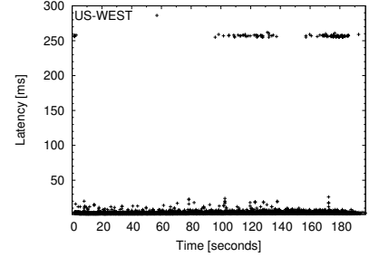
(c) Latency of individual operations of US-W datcenter (ad counter application).
