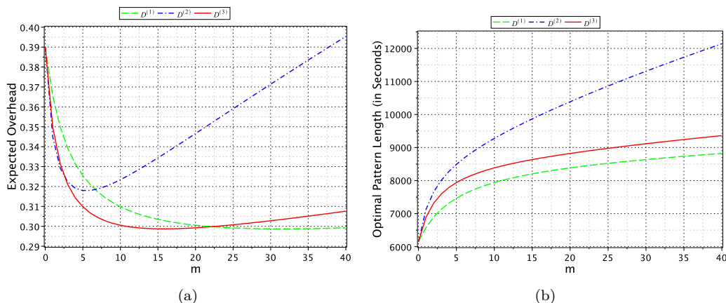
Figure 2: Expected overhead (a) and optimal length (b) of a pattern against the number of partial verifications when a single type of detector is used for three different detectors. The costs and recalls of the three detectors are V^{(1)} = 3 seconds, V^{(2)} = 30 seconds, V^{(3)} = 6 seconds, and r^{(1)} = 0.5 , r^{(2)} = 0.95 , r^{(3)} = 0.8 . The costs of checkpointing and guaranteed verification are C = V^* = 600 seconds. The platform MTBF is \mu = 31536 seconds.
