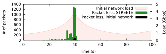
Fig. 10: Packet loss.
