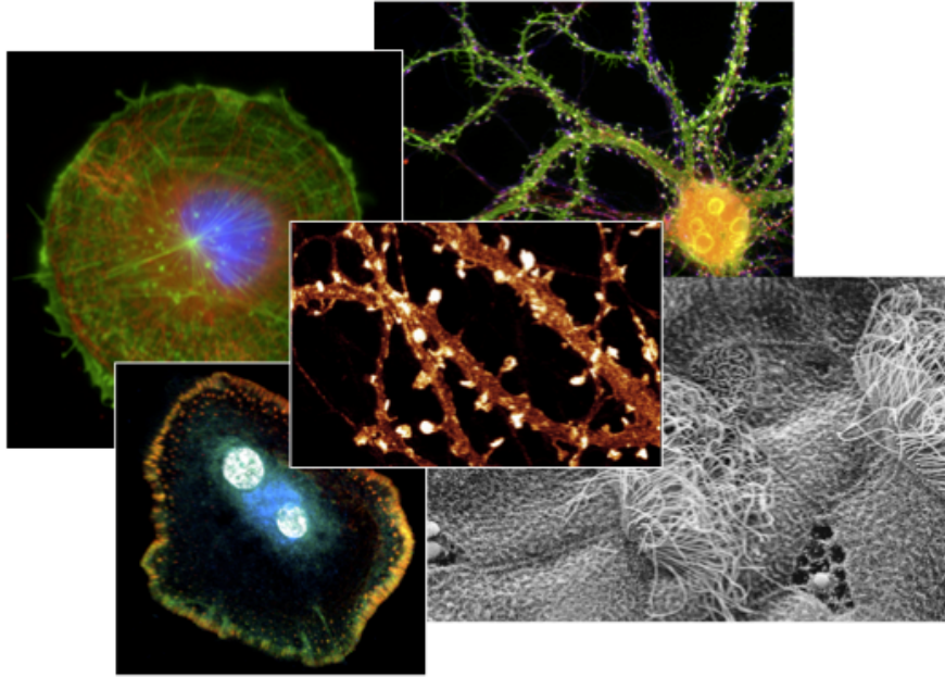
FIGURE 1 – An illustration of microscopy modalities used for investigation in cell biology at the sub-cellular and cellular scales (by courtesy of france-bioimaging.org)
