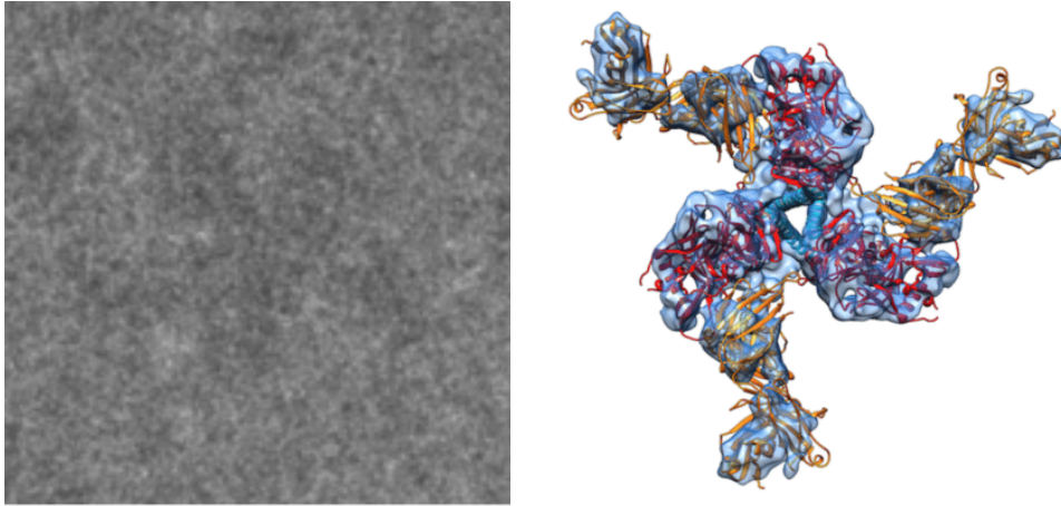
FIGURE 2 – Left : Example of a projection of HIV-1 envelope glycoprotein as seen at the electron Microscope. Right : corresponding 3D reconstruction at 6Å resolution from several thousands of such projections [41].
