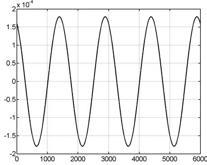
Figure 2: \Gamma(\tau, \zeta(0)) - \Gamma(\tau, \zeta_\tau(0)) as a function of \tau .
