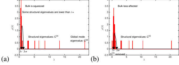
Fig. 3. Example of the distribution of the eigenvalues of \mathbf{C} , (a) when there is a global mode and the bulk is squeezed and is not located in the interval [\lambda_-, \lambda_+] (2 isolated eigenvalues that should be in \mathbf{C}^{(s)} are lower than \lambda_+ , and (b) after filtering of the global mode (the interval [\lambda_-, \lambda_+] is more representative of the bulk).
