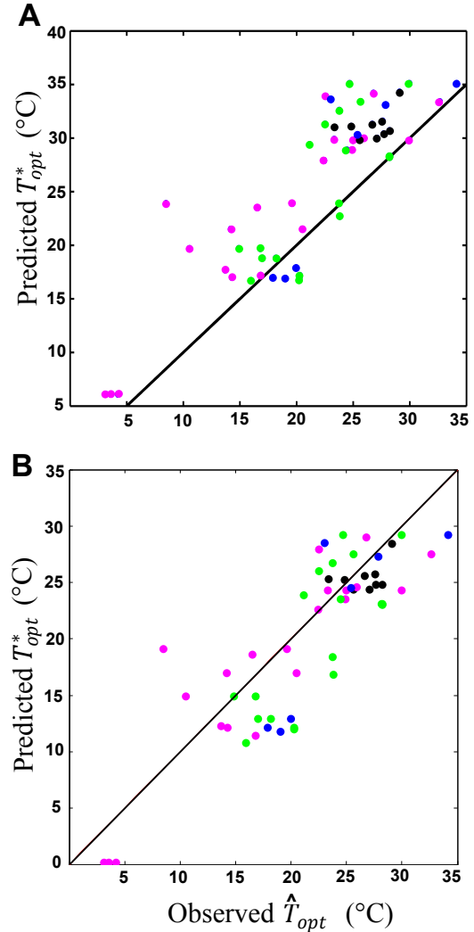
Fig. 4. Predicted T_{opt}^* compared to experimental \hat{T}_{opt} for Eppley-Norberg model (A) and Bernard and Rémond model (B). Phytoplankton phylogenetic groups are indicated in color in (B): green, Dinoflagellates, pink, Diatoms, black, Cyanobacteria, blue, others.
