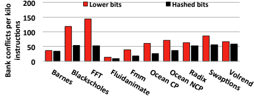
Figure 7: Bank conflicts for 4W \times 4T DITVA
