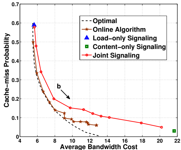
Figure 3: Performance curves.
