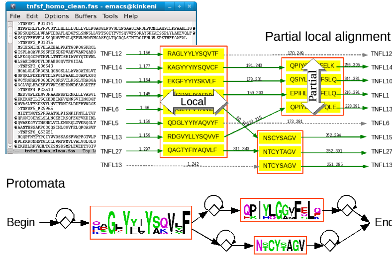
Fig. 10 Learning automata by partial local alignment from set of protein sequences.
