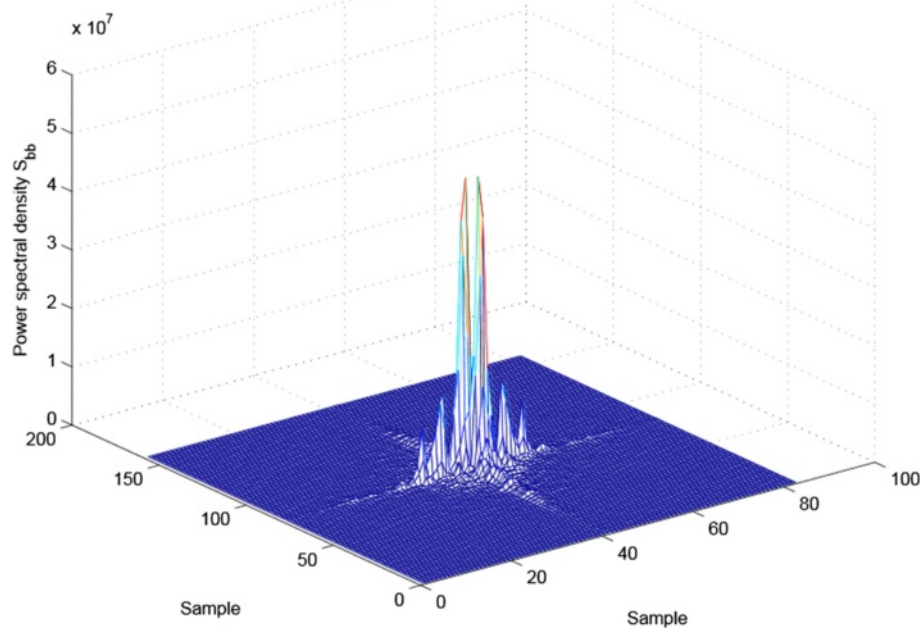
Fig. 9 The power spectral density of the extracted 2D deterministic shadowing from the MR-FDPF model
