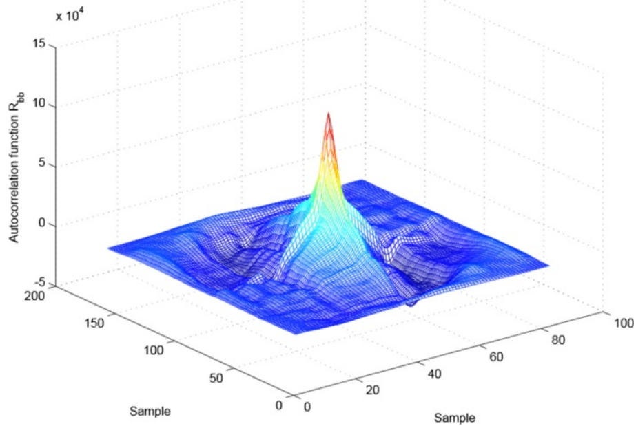
Fig. 8 The autocorrelation function of the extracted 2D deterministic shadowing from the MR-FDPF model
