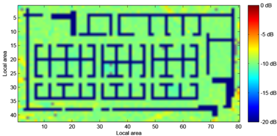
Fig. 5 The estimated m parameter map of the Nakagami- m fading with goodness of fit test
