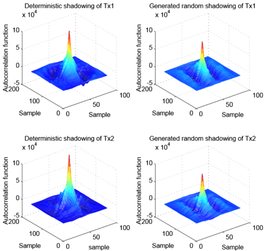
Fig. 13 The autocorrelation function comparison of the extracted 2D deterministic shadowing from the MR-FDPF model and the generated 2D correlated random shadowing
