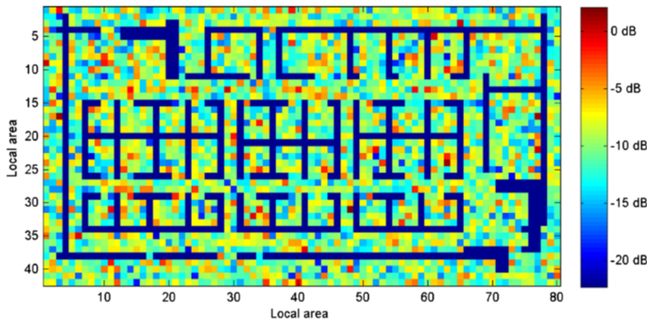
Fig. 10 The generated 2D random shadowing with cross-correlation
