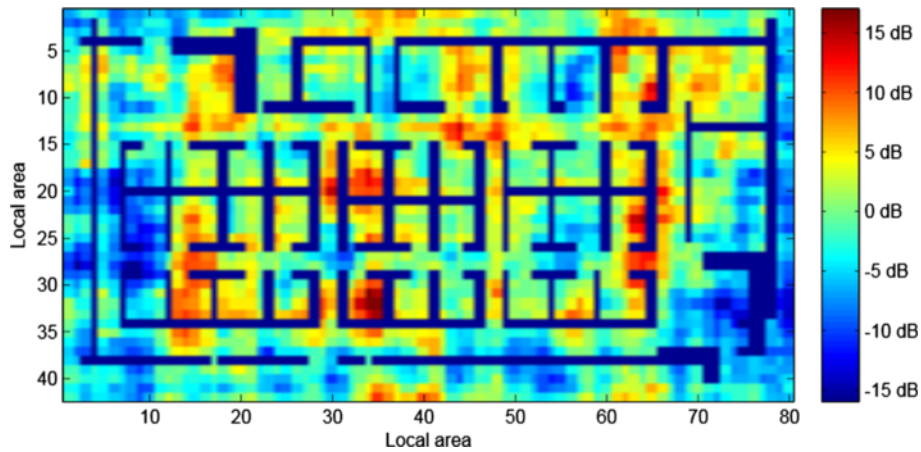
Fig. 12 The generated 2D random shadowing with both the cross-correlation and the spatial correlation
