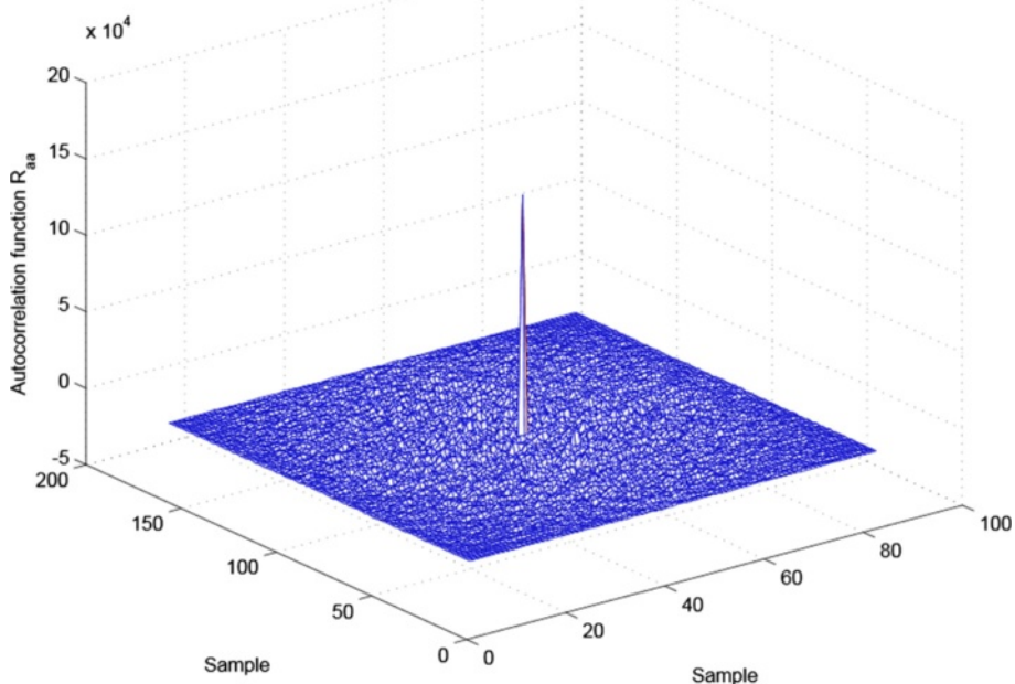
Fig. 11 The autocorrelation function of the generated 2D random shadowing with cross-correlation
