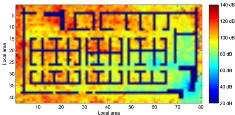
Fig. 14 The generated 2D semi-deterministic path loss for Tx1
