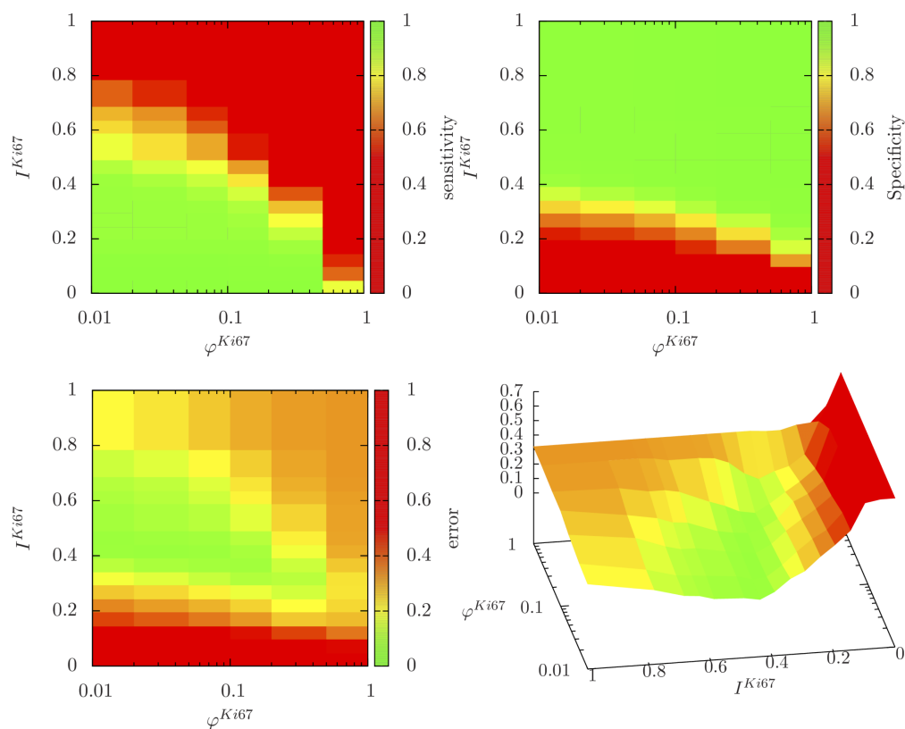
Figure 14. Sensitivity analysis for threshold parameters I^{Ki67} and \varphi^{Ki67} . The plots show the sensitivity, specificity and classification error comparing the manual detection with the automated detection for a combination of \{I^{Ki67}, \varphi^{Ki67}\} .
