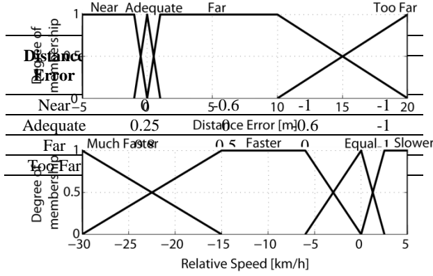
Fig. 3. Membership functions for CACC controller inputs.
