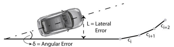
Fig. 5. Input variables defined for lateral control.
