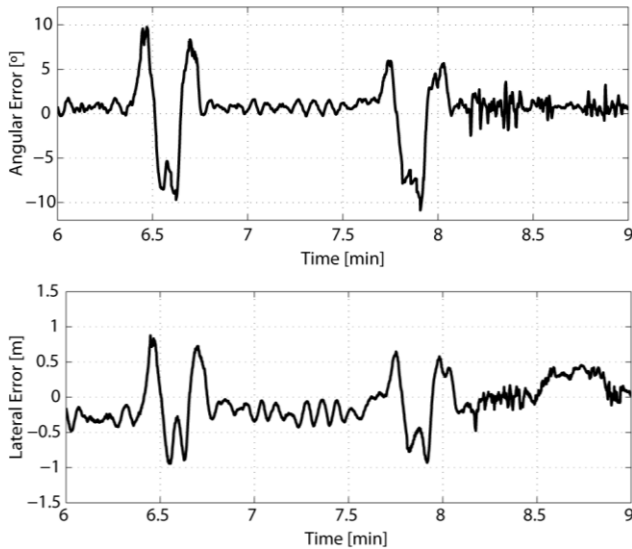
Fig. 14. Evolution of the input variables for lateral control. Upper image: Angular error. Bottom image: Lateral error.
