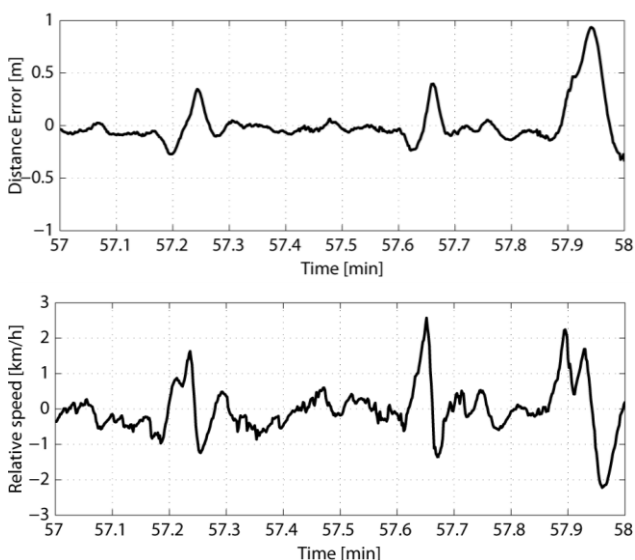
Fig. 18. Evolution of the input variables for longitudinal control in the motorway scenario. Upper image: Distance error. Bottom image: Relative speed.
