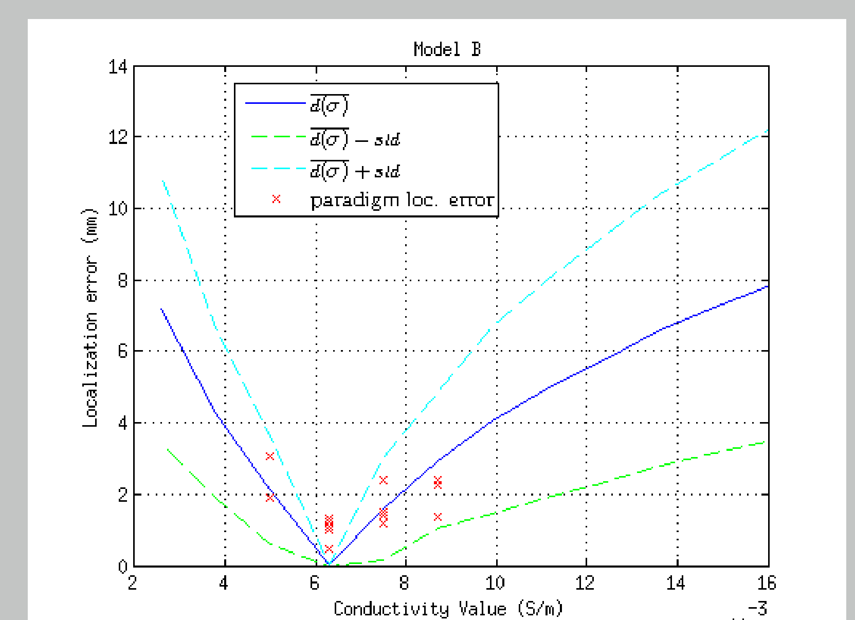
Figure 1 : Plot of localization errors across evenly spread conductivity values for the two test models. The red x symbols indicate the localization error for the 20 manually selected paradigms. The blue line indicates the mean localization errors for 1000 randomly placed sources.
