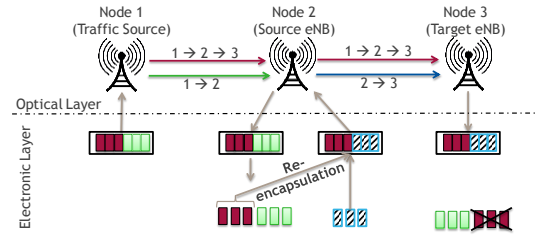
Fig. 3: Electronic forward with re-encapsulation
