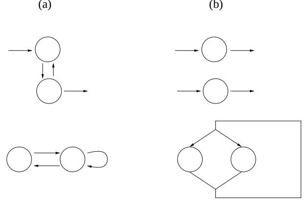
Fig. 5. A mixed queueing network consisting of an open subnetwork and a closed subnetwork (a) and the corresponding network with the same arrival rates, no routing for the open subnetwork and homogeneous routing probabilities for the closed subnetwork (b).
