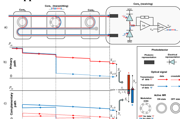
Figure 1. Transmission of data ‘1’ and ‘0’ through primary and complementary paths respectively.
