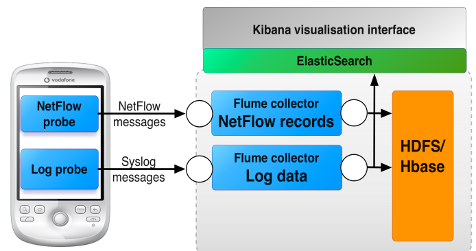
Fig. 1. Architecture and details of the collection and analysis platform.
