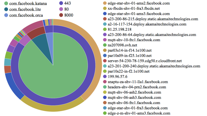
Fig. 2. A piechart of the communication patterns of the Android version of Facebook application.
