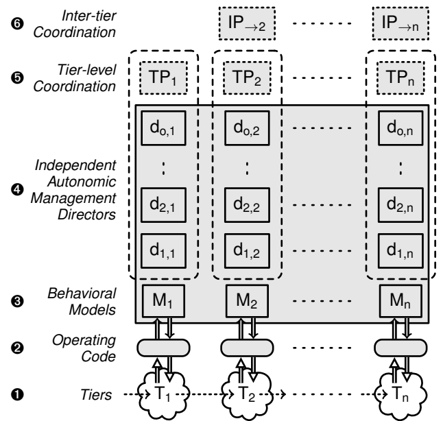
Fig. 5. Principle of the approach for the management of an n -tier application. “ \rightarrow ” represent service requests. Dotted areas depict synchronous nodes encoding predicates. A dashed area encompassing tier-level coordination predicate TP_i also covers the directors it controls. Plain areas represent synchronous nodes controlled by a synthesized coordination controller. Most synchronous signals have been omitted to ease readability.
