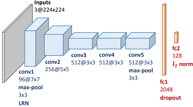
Figure 2: Our network architecture for pose embedding. The network consists of 5 convolution layers (conv) followed by 2 fully-connected layers (fc). In details, Local Response Normalization (LRN) [31] is applied after conv1, and the output of fc1 is regularized by Dropout [44]. All the convolution layers and related operations ( blue ) are transferred directly from those of the VGG-S network [10], and their parameters are fine-tuned during training.
