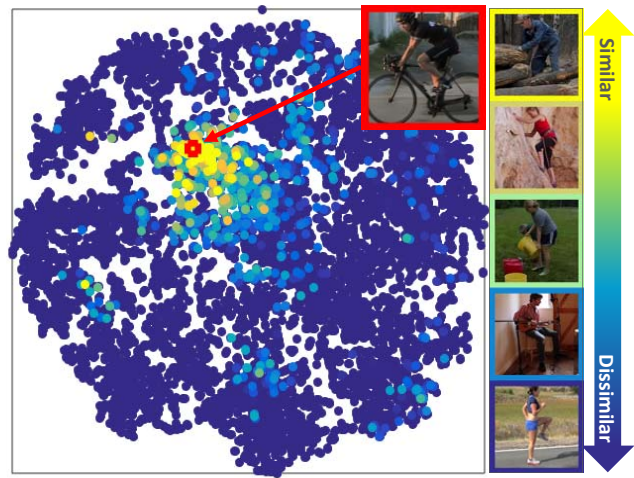
Figure 1: The manifold of our pose embedding visualized using t-SNE [51]. Each point represents a human pose image. To better show correlation between the pose embedding and annotated pose, we color-code pose similarities in annotation between an arbitrary target image (red box) and all the other images. Selected examples of color-coded images are illustrated in the right-hand side. Images similar with the target in annotated pose are colored in yellow, otherwise in blue. As can be seen, yellow images lie closer by the target in general, which shows that a position on the embedding space implicitly represents a human pose. (Best viewed in color.)
