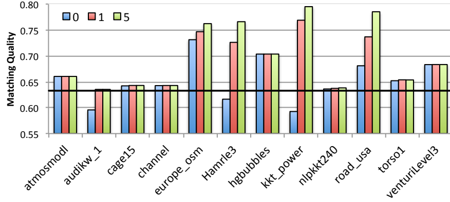
(a) ONEsIDEDMATCH
