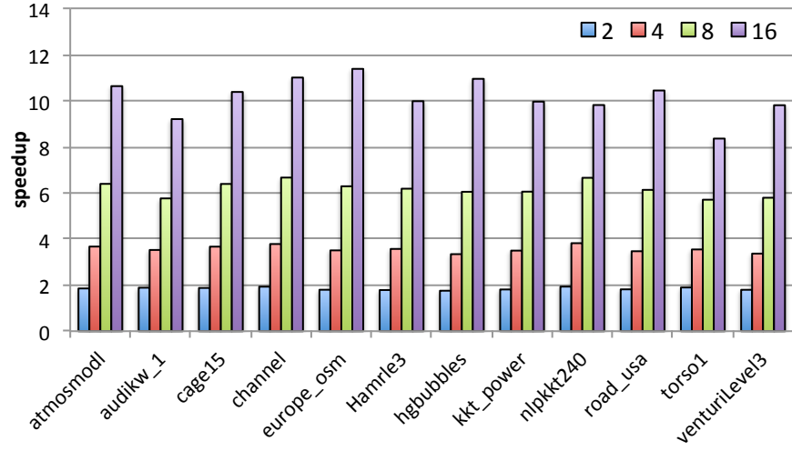
(b) ONESIDEDMATCH
