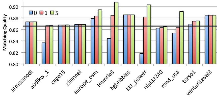
(b) TwOSIDEDMATCH
