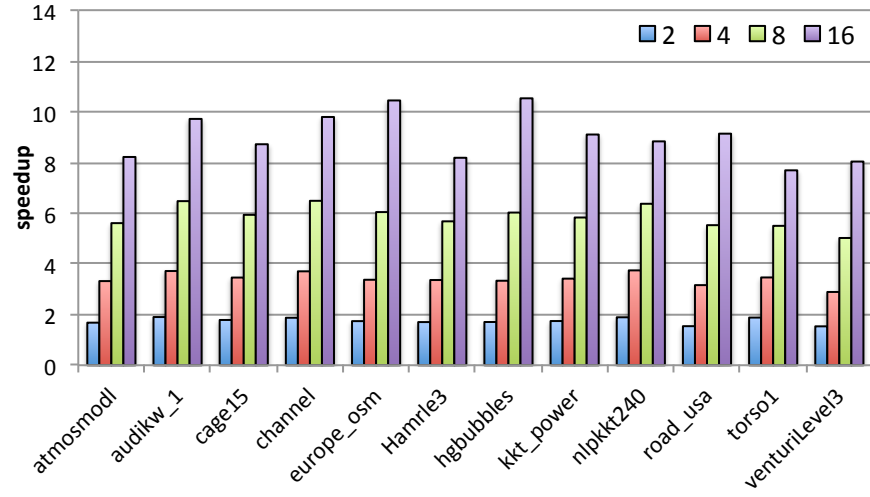
(a) SCALESK
