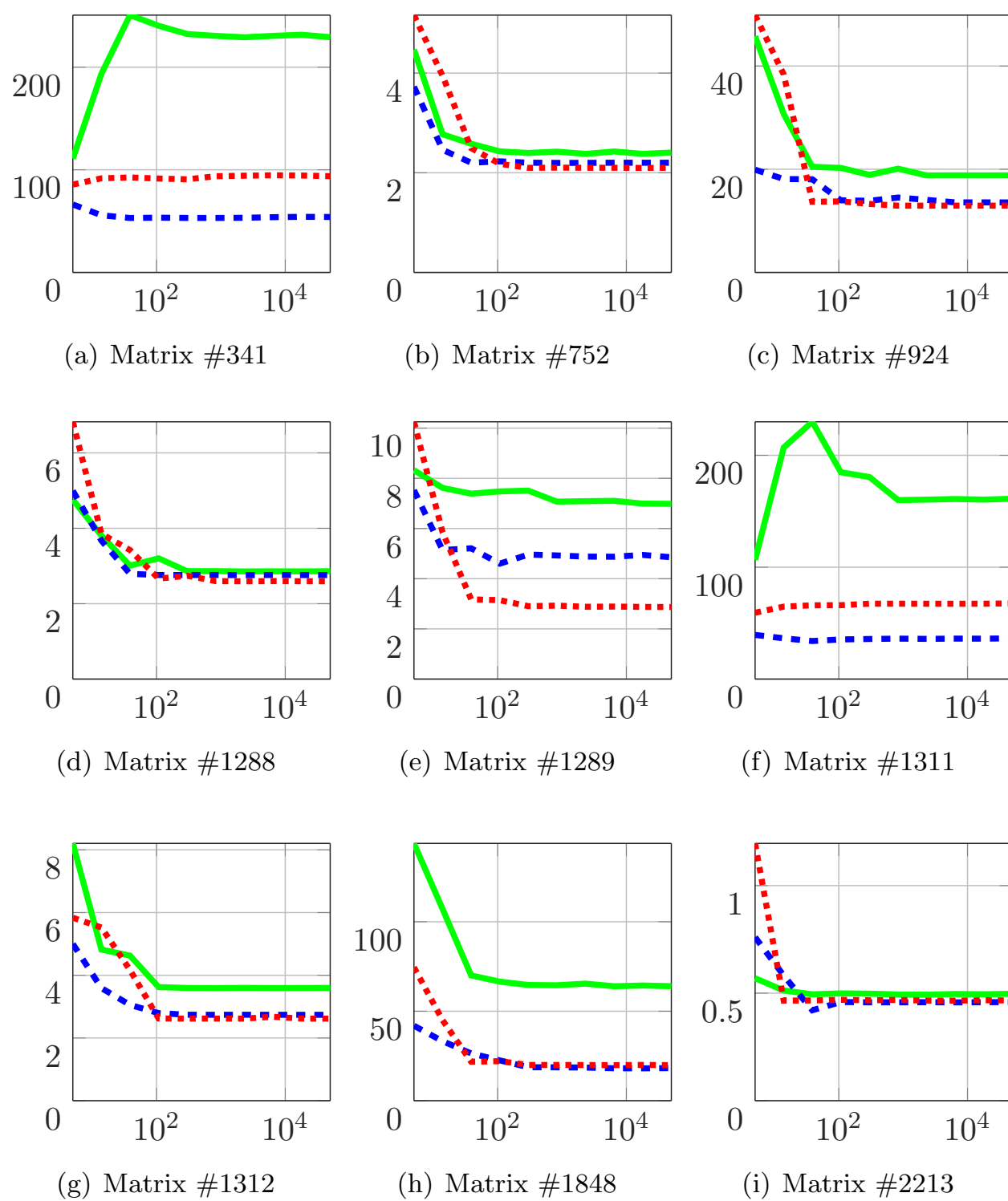
Figure 1: Execution time in seconds ( y axis) of ONLINE-DETECTION (dotted), ABFT-DETECTION (solid green line) and ABFT-CORRECTION (dashed blue) with respect to the normalized MTBF ( x -axis). The matrix number is in the subcaption.
