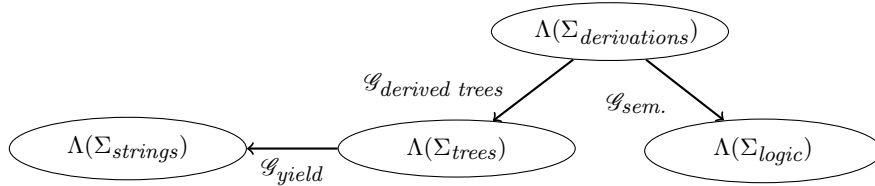
Figure 12: ACG composition for control and syntax-semantic interface
