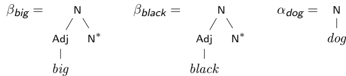
Figure 23: TAG elementary trees for adjectives
