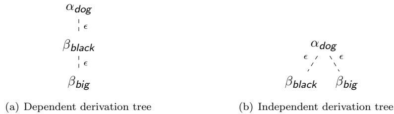
Figure 25: Alternative notions of derivation trees
