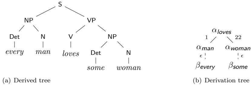
Figure 22: TAG analysis of every man loves some woman
