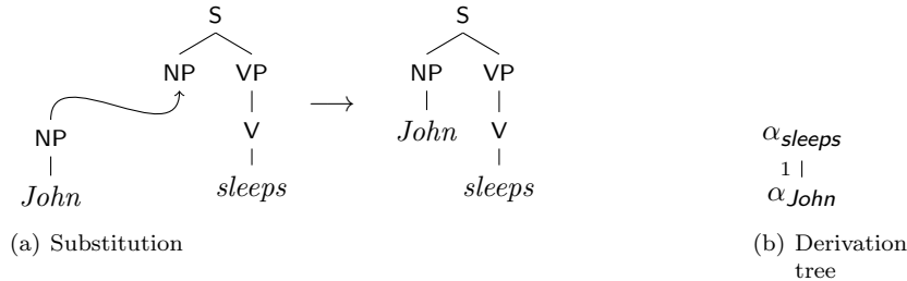
Figure 2: Substitution operation
