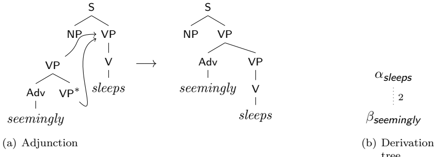
Figure 3: Adjunction operation
