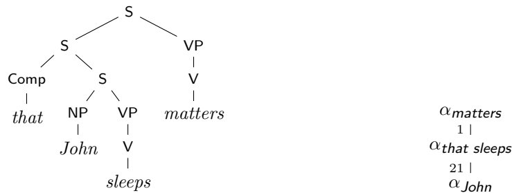
(a) Derived tree for that John sleeps matters (b) Derivation tree for that John sleeps matters
