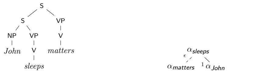
(a) Syntactic tree which is not a TAG derived tree (b) Forbidden corresponding derivation tree
