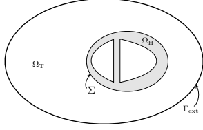
Fig. 1. Two-dimensional geometrical description: heart domain \Omega_H , torso domain \Omega_T (extramycardial regions), heart-torso interface \Sigma and torso external boundary \Gamma_{ext} .
