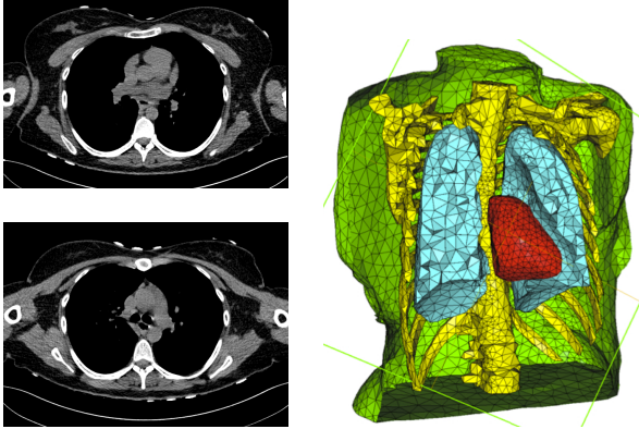
Fig. 2. Two slices of the CT-scan images (left). Torso geometry showing the epicardium (heart-torso interface \Sigma ) (red), lungs (light blue), bones (yellow) and torso external boundary \Gamma_{ext} (green).
