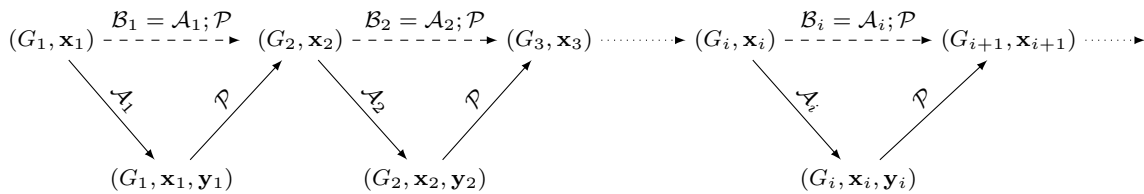
Fig. 1 Schematic view of an alternating algorithm for (\mathcal{A}_i)_{i \in \mathbb{N}} and \mathcal{P} .
