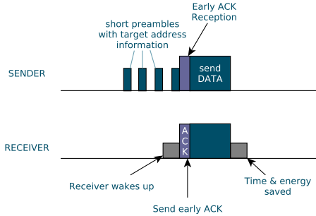
Figure 1: X-MAC short preamble approach.
