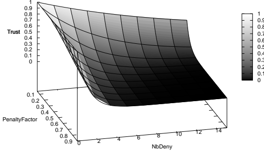
Fig. 3: Trust assessment function.
