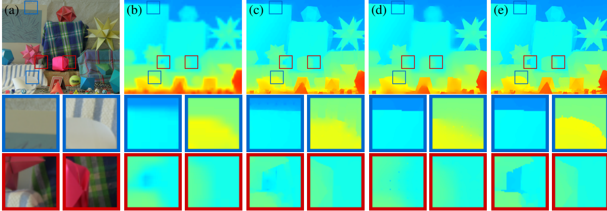
Figure 1. Comparison of static and dynamic guidance regularization methods. Given (a) a HR color image, (b) a LR depth map is upscaled ( \times 8 ) by our model using (c) static guidance only, (d) dynamic guidance only, and (e) joint static and dynamic guidance. See Sec. 4.1 for details. (Best viewed in color.)
