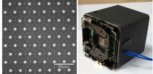
Figure 3. Left: Image of the micro-lens array taken with a microscope with top illumination. We can see the hexagonal structure of the micro-lens array. The bright dot in the middle of each hexagon is an image of the light source reflected by the surface of the micro-lens. Right: The Lytro camera without its optics.
