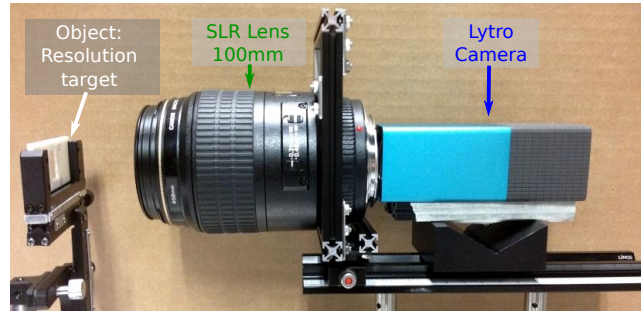
Figure 12. Setup from the SLR + Lytro experiment using a 100mm SLR lens (100mm SLR + Lytro).
