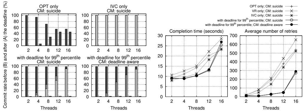
(c) synquake : Execution modes and success of committing by the deadline. (d) synquake : Completion time for the complete workload and contention.
