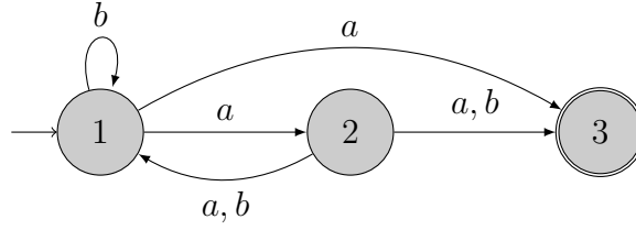
Automaton in \mathfrak{N}(3)^\bullet , \mathfrak{N}_4(3)^\bullet , \mathfrak{N}'_2(3)^\bullet and in \mathfrak{N}(3) , \mathfrak{N}_4(3) , \mathfrak{N}'_2(3) .
