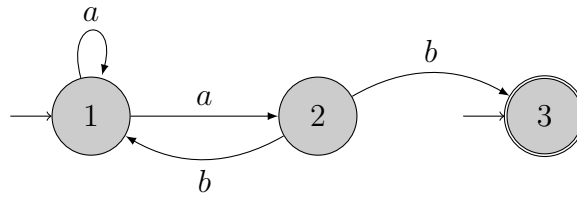
Automaton in \mathfrak{N}(3) , \mathfrak{N}_2(3) and \mathfrak{N}'_2(3) but not in any dotted class.
