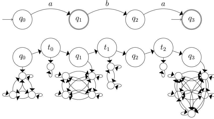
Figure 4: Example \mathcal{A} and G_{\mathcal{A}} , h(a) = 1 and h(b) = 2
