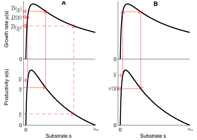
Fig. 2. How to choose D in one region (see Section V-A). A, thin lines: one can choose any D \in (\underline{D}(\bar{y}), \overline{D}(\underline{y})) ; dashed lines: it is impossible to fulfill Conditions (5-6), given that \underline{D}(\bar{y}) > \overline{D}(\underline{y}) ; B: \psi(\bar{y}) represents the lower bound for \underline{y} (limit case).
