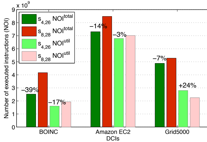
(a) Differences in total and utilizable number of executed instructions.
