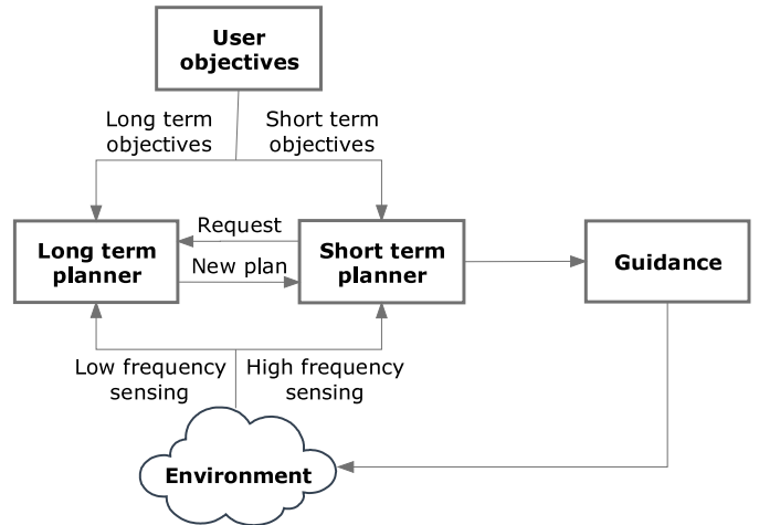
Fig. 1. Diagrammatic overview of the motion planning framework. The whole process can be divided into three main elements: the long term planner that considers the long term objectives, the short term planner that optimises the long term plan taking into account the short term objectives and constraints, and the guidance that drives the robot towards the goal.
