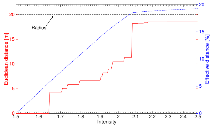
Fig. 12. The effect of intensity on the minimum Euclidean distance from a path to an undesirable zone on a particular simulation run. As the intensity increases the path is pushed away from the undesirable location (the Euclidean distance increases) until it approximates the specified radius (20 m, dashed line). The constraint is actually implemented with respect to the effective length of the path, which is shown for comparison.
