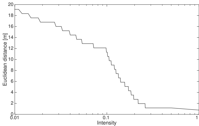
Fig. 11. The effect of intensity on the minimum Euclidean distance from a path to a desirable zone on a particular simulation run. As intensity increases the path is attracted towards the desirable location: the Euclidean distance decreases.
