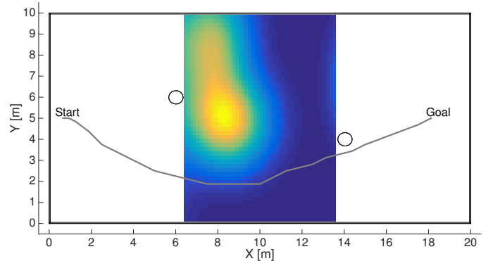
Fig. 7. Simulation with a heat map. The path computed by the planner is represented by the continuous line and bypasses the crowded region in the middle of the map (i.e., yellow area). The preference is for cold zones (i.e., blue-coloured areas).
