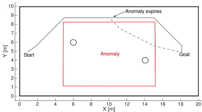
Fig. 8. Simulation with anomalies: two independent simulations are shown. The dashed line represents the path generated when the anomaly is set to expire half way to the goal. The continuous line, instead, shows the resulting path when the anomaly does not expire.
