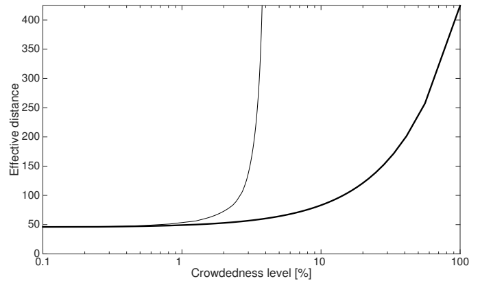
Fig. 10. Relation between level of crowdedness and effective length of the path. When the planner is aware of the heat maps in the environment, the long term planner is able to avoid the heat and the effective distance increases slowly with increasing crowdedness (thick line). Without this information, the long term planner just chooses the shortest Euclidean path, whose effective length increases exponentially.
