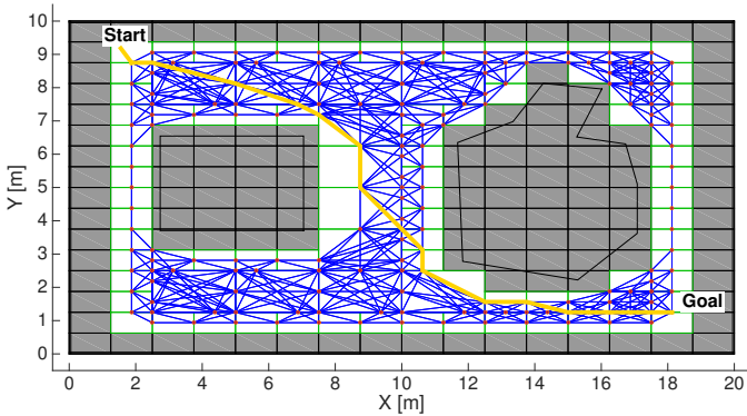
Fig. 5. Graph and a sample path generated from the map depicted in Figure 4.
