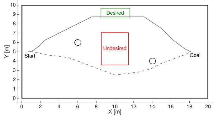
Fig. 6. Simulation with constraints. The picture shows two independent simulations of how the planner deals with desirable and undesirable zones. The continuous line is the result of the constraint “stay close to the desirable zone” and “stay away from the undesirable zone”, while the dashed line addresses only the latter.
