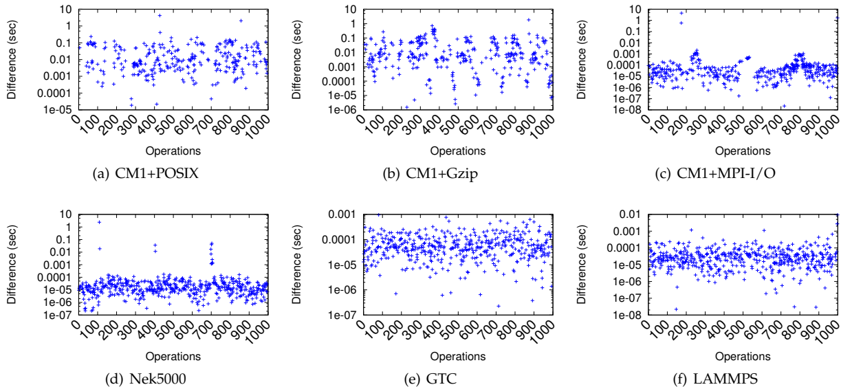
Fig. 8: Difference between predicted and observed interarrival times of I/O events.
