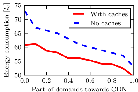
(c) Germany
