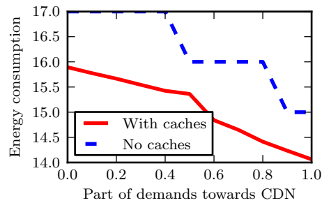
(a) Atlanta
