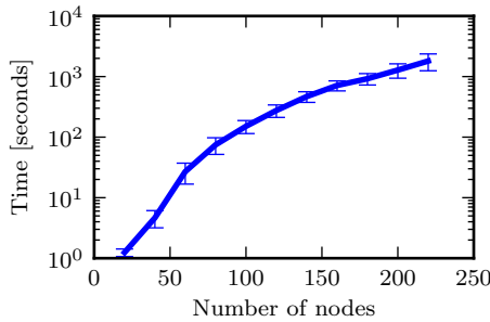
(b) Execution time (note the log scale)
