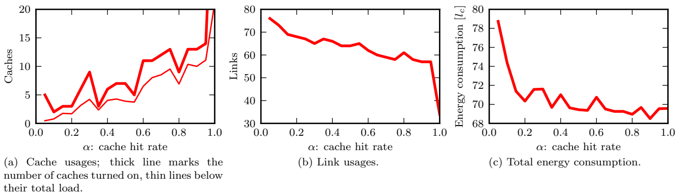
FIGURE 3: Results as a function of parameter \alpha (cache hit rate) for Germany50 . Power consumption is reported with a normalized unit equal to the power used by a network link.
