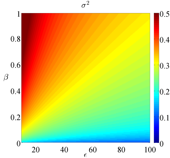
Figure 3: The level of phenotypic diversity depends on the rate of epimutations and the strength of natural selection. Plot of the level of phenotypic diversity \sigma^2 as a function of the strength of natural selection \epsilon and the rate of epimutations \beta . Further technical details of the numerical solutions are provided in Appendix B.
