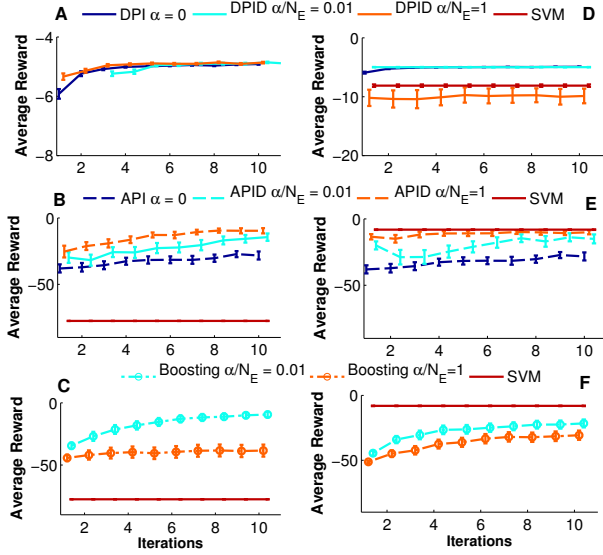
Figure 4: Panel A: DPI versus DPID when fixing N_E = 15 optimal expert demonstrations and increasing N_{RL} by 500 at every iteration. Panel D: DPI versus DPID when fixing N_E = 100 sub-optimal expert demonstrations and increasing the RL data by 500 at iteration (0.5 prob. of wrong action). Panels B/E and C/F: Same as A and D for API/APID and RLED respectively.
