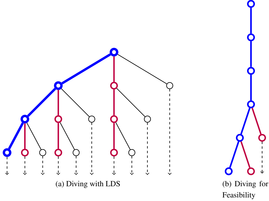
Figure 2: (a) is a “Diving with LDS” example for \maxDepth = 3 and \maxDiscrepancy = 2 ; (b) is a “Diving for Feasibility” example for \maxDiscrepancy = 1 , assuming a feasible solution was found after 2 back-tracks
