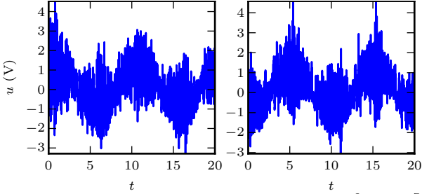
Fig. 10: Control inputs for two values of the gain: 10^{-2} and 10^7 and with a sampling period of 10ms.
