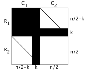
Fig. 2. A generic full-sprank matrix structure that is bad for KS.
