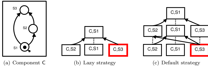
Figure 5: Difference between lazy and default strategies.
