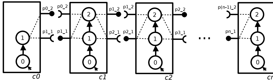
Figure 10: Component types for the validation with artificial instances.
